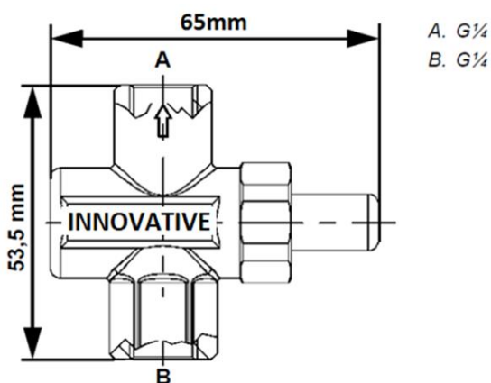
Push Button Stop Valve G 1/4"
