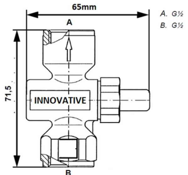
Push Button Stop Valve G 1/2"
